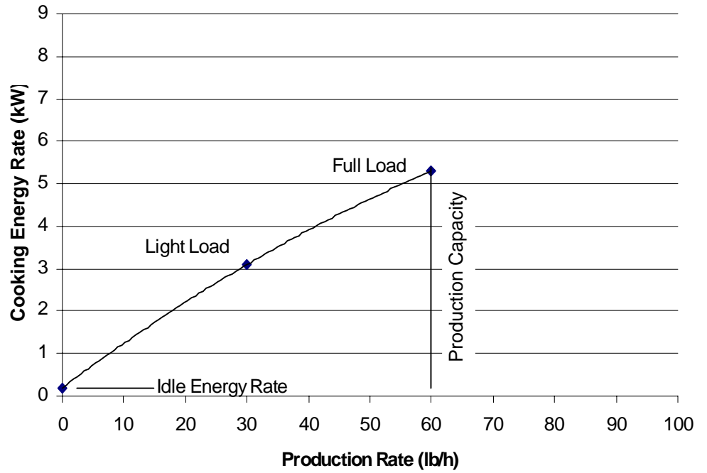
Figure 3-6. Steamer Cooking Energy Consumption Profile, Green Peas, Low Power.
