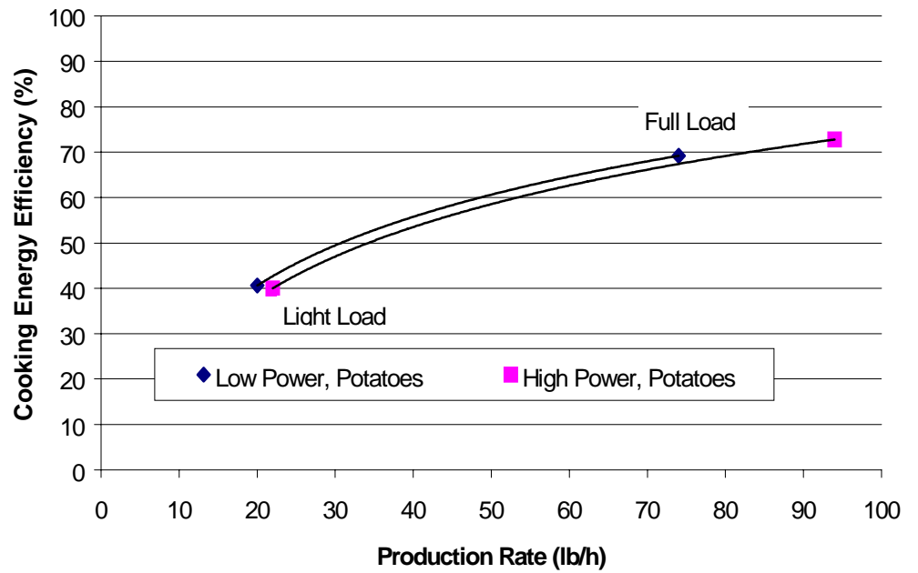
Figure 3-5. Steamer Part-Load Red Potato Cooking Efficiency.
