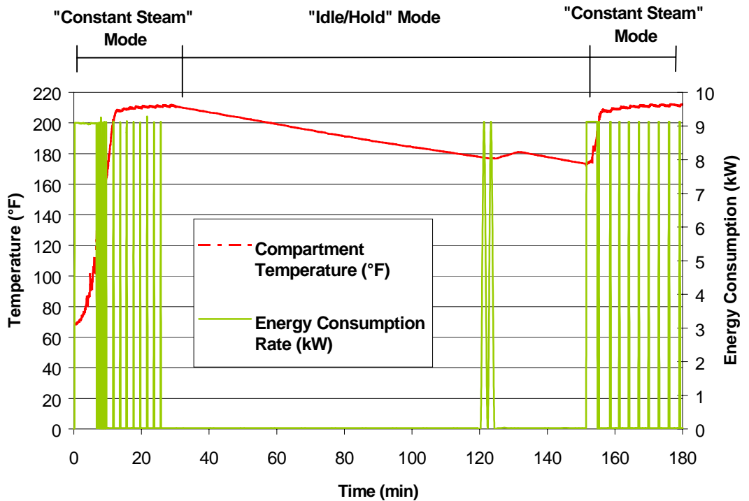
Figure 3-1. Preheat and Idle Characteristics.
