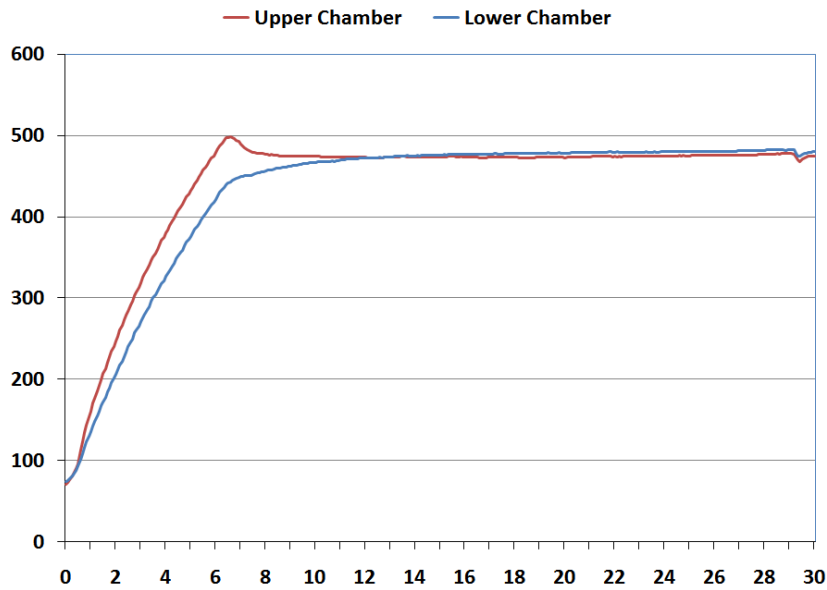
Preheat Curve
