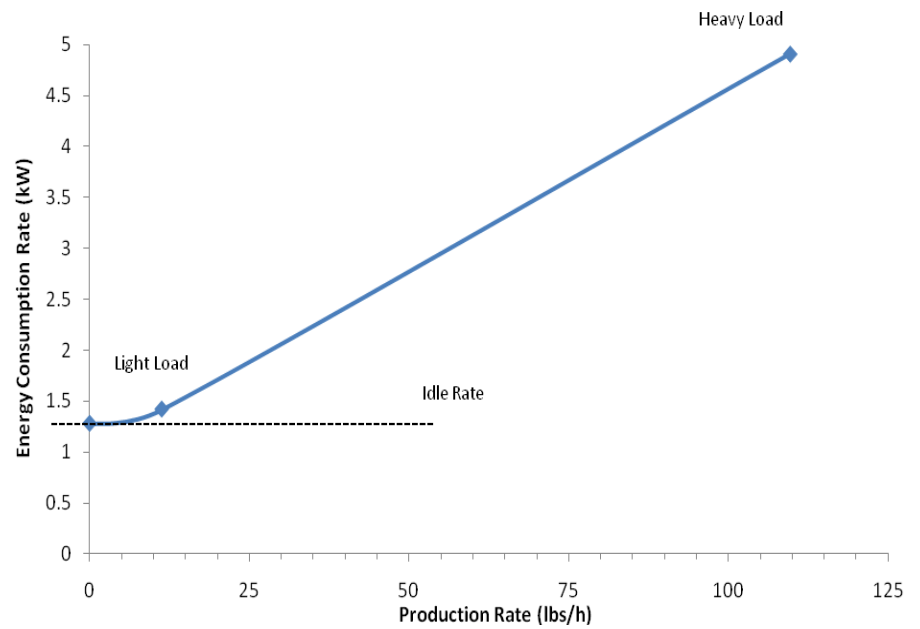
Figure 3-5. Electric cooking-energy consumption profile.
