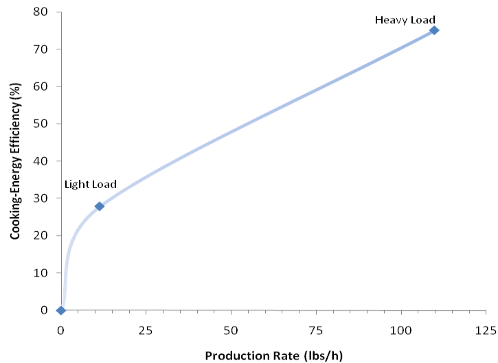
Figure 3-4. Deck oven part load cooking energy efficiency.
