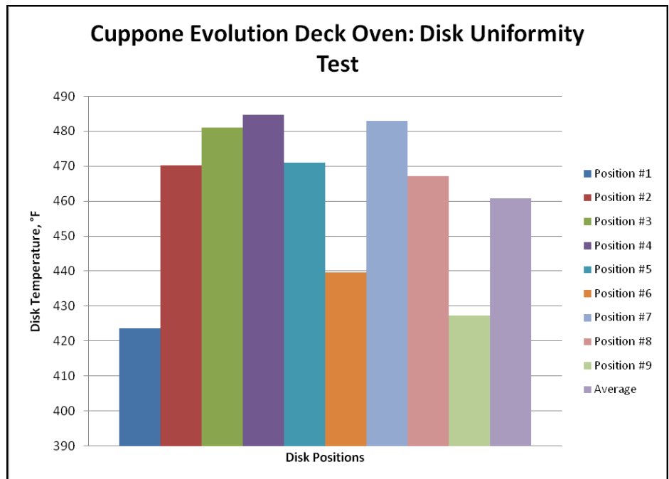
Figure 3-2. Disk Uniformity temperature graph.
