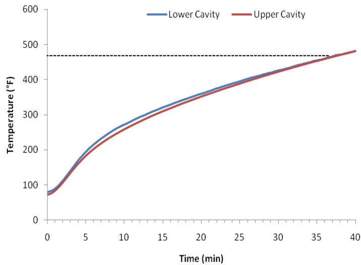
Figure 3-1. Preheat characteristics.
